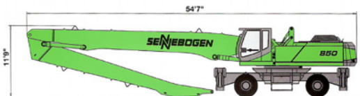
850 M with Boom 39'8" and Stick 31'5"
